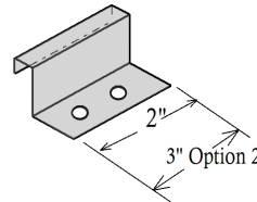
26ga Stainless Steel clip
